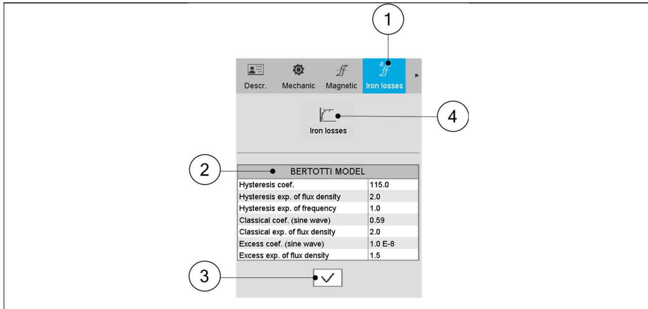
Definition of iron loss coefficients
