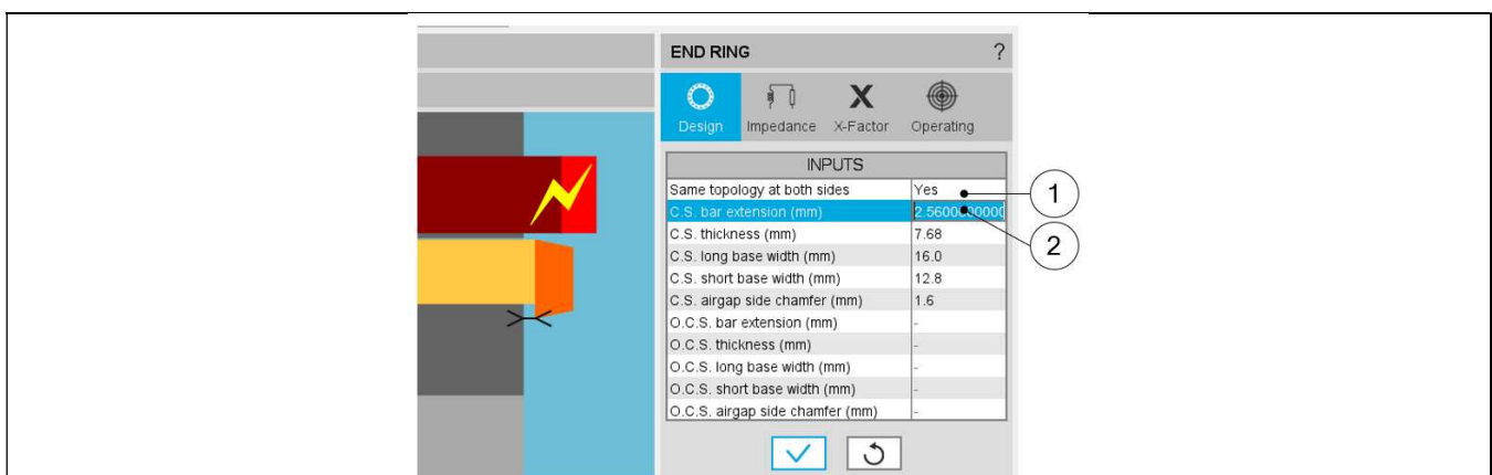
END RING - DESIGN – design area
