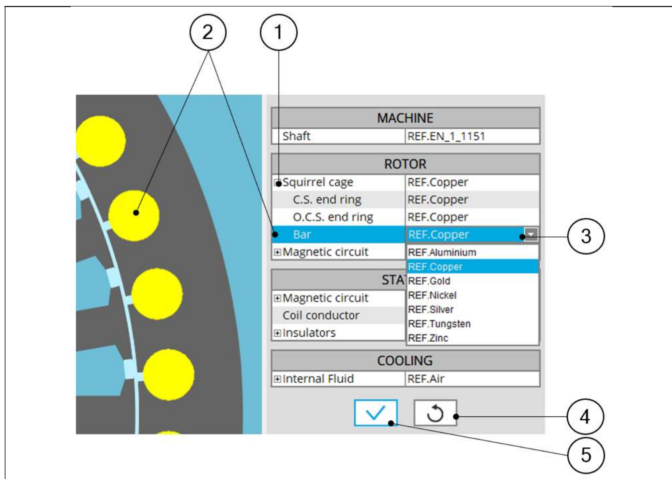
Assign Materials to BARS in the rotor
