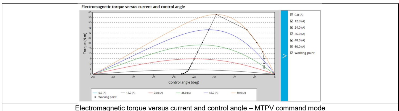
Electromagnetic torque versus current and control angle – MTPV command mode
